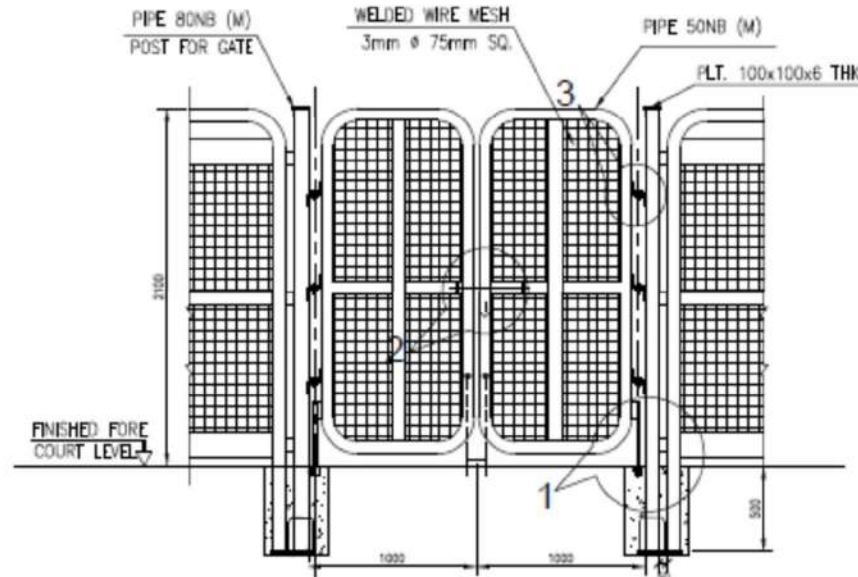
2.0M WIDE GATE DETAIL
