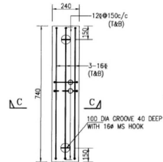
RCC DETAIL OF PRECAST SLAB
