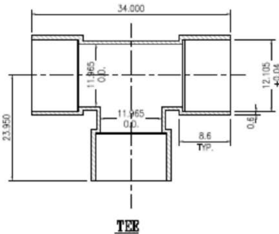
FITTING AS PER EN 1254 PART-1
