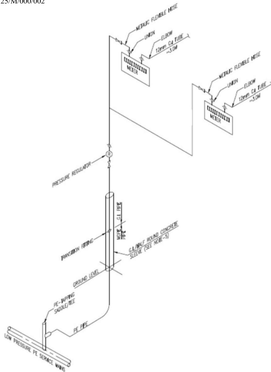
SINGLE REGULATOR & DOUBLE CONNECTION ON GROUND FLOOR
