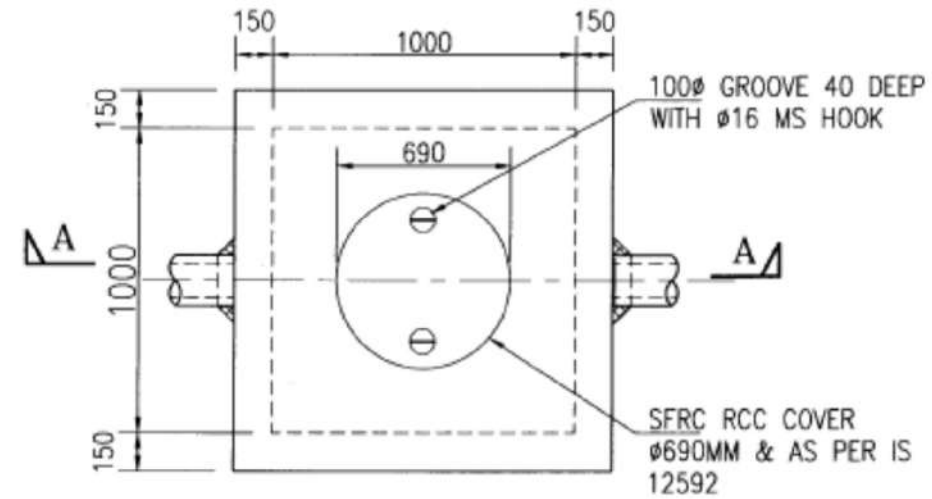
PLAN OF VALVE PIT VP-1
