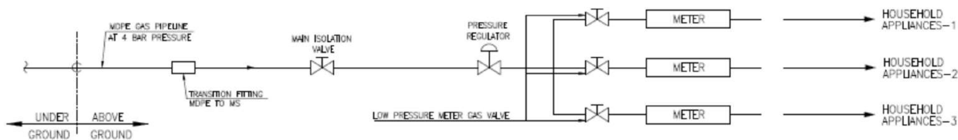
SCHEME OF NATURAL GAS SUPPLY TO DOMESTIC CONSUMERS
