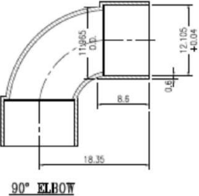
FITTING AS PER EN 1254 PART-1
