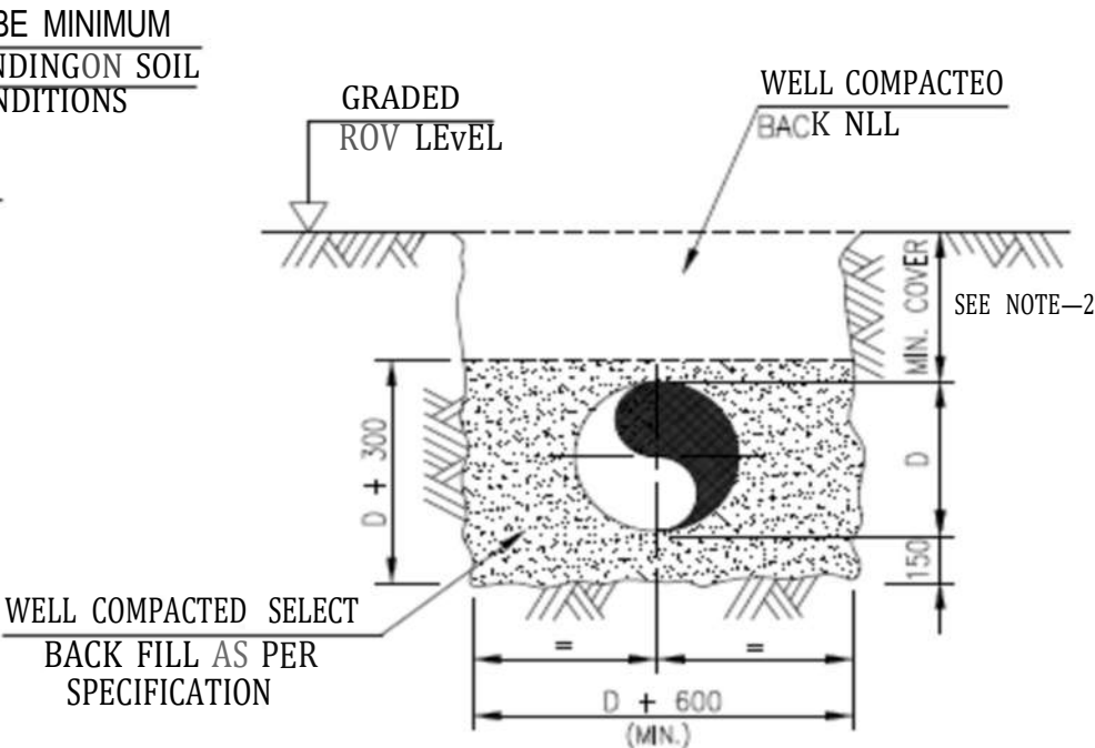
TRENCH IN CONSOLIDATED ROCK TYPICAL SECTION
