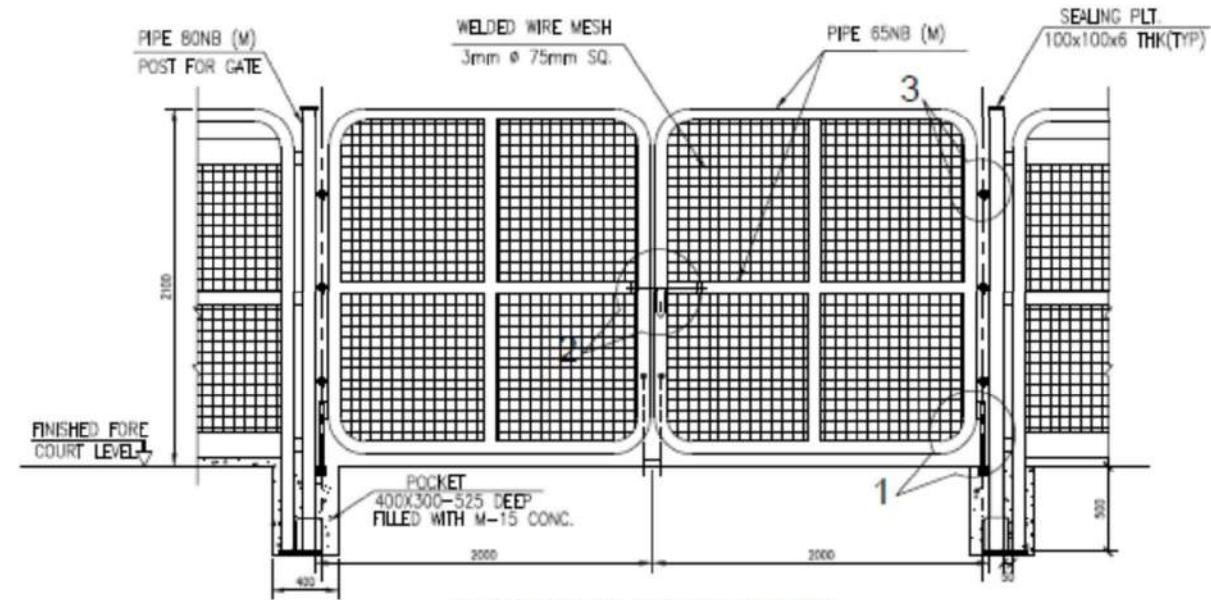
4.0M WIDE GATE DETAIL
