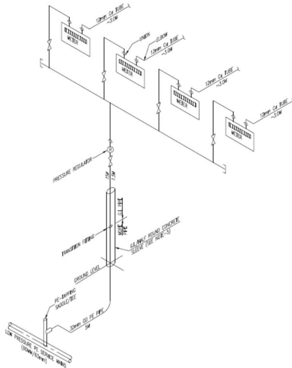
FOUR CONNECTION ON GROUND FLOOR
