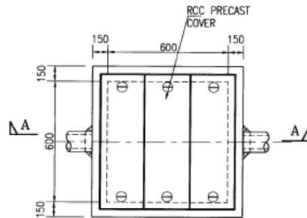
PLAN OF VALVE PIT
