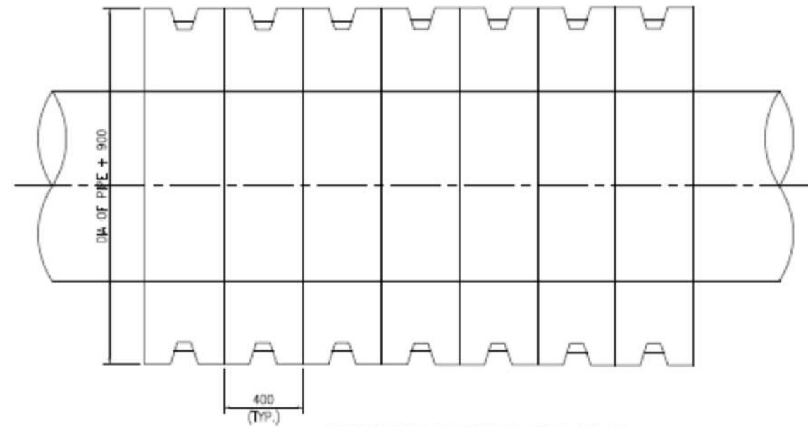
PROTECTIVE CONCRETE SLAB PLAN
