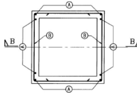
REINF. DETAIL OF VALVE PIT
