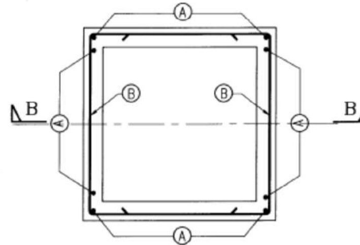
REINF. DETAIL OF VALVE PIT
