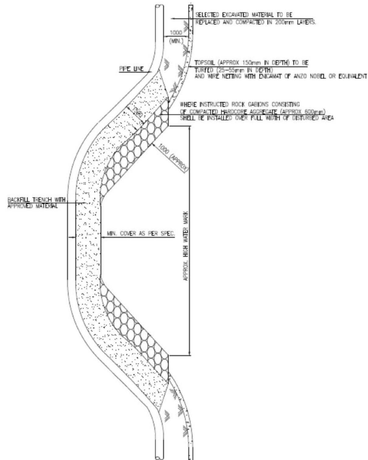
STD. DETAIL OF BACKFILL FOR DRAIN CROSSING
