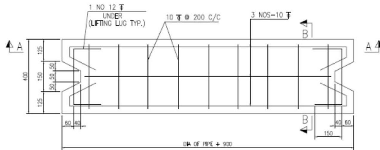
REINF. DETAIL PROTECTIVE CONCRETE SLAB
