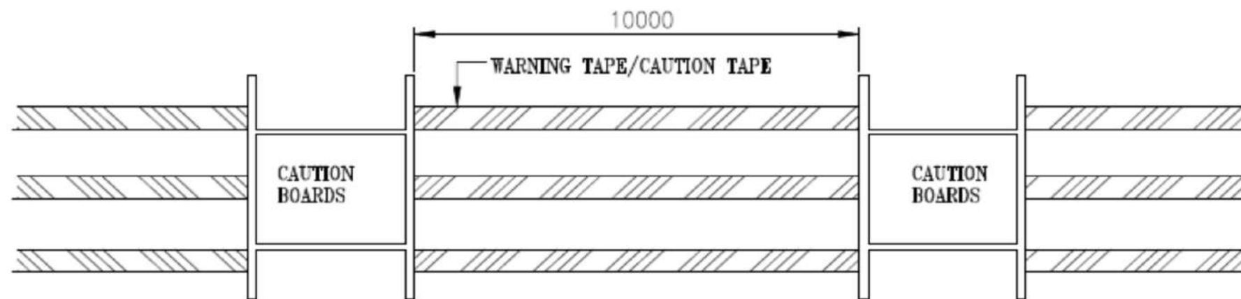
SCHEMATIC LAYOUT OF CAUTION BOARDS AND BARRICADDING
