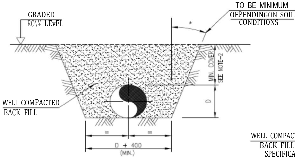
TRENCH IN NORMAL SOIL TYPICAL SECTION
